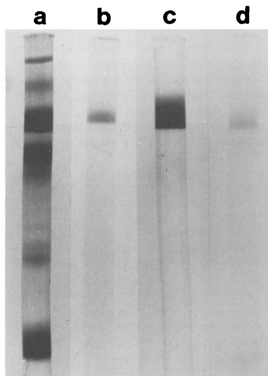
Fig.2. SDS-gel electrophoresis. Samples applied to the gels were: whey protein, 120 \mu\text{g} (a); isolated lactoferrin, 8 \mu\text{g} (b); 60 \mu\text{g} (c,d). Gels a-c were stained for protein with Coomassie blue and gel (d) with the periodic acid-Schiff reagent for carbohydrate. Samples were treated with 2-mercaptoethanol prior to application. The gels were 60 \times 7 mm and the current 8 mA/tube. Migration was towards the anodic end (the lower part of the photograph).
