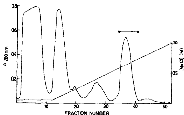
Fig.1. Heparin-Sephacrose chromatography of human whey. Whey (50 ml) dialyzed against 0.05 M NaCl in 5 mM veronal-HCl, (pH 7.4) was applied to the column (10 ml settled gel). The column was washed with 50 ml of the same buffer and then eluted with a linear gradient of NaCl (400 ml) as indicated. The flow rate was 52 ml/h. Fractions 34-42 (total vol. 78 ml) were combined and used for further analysis.
